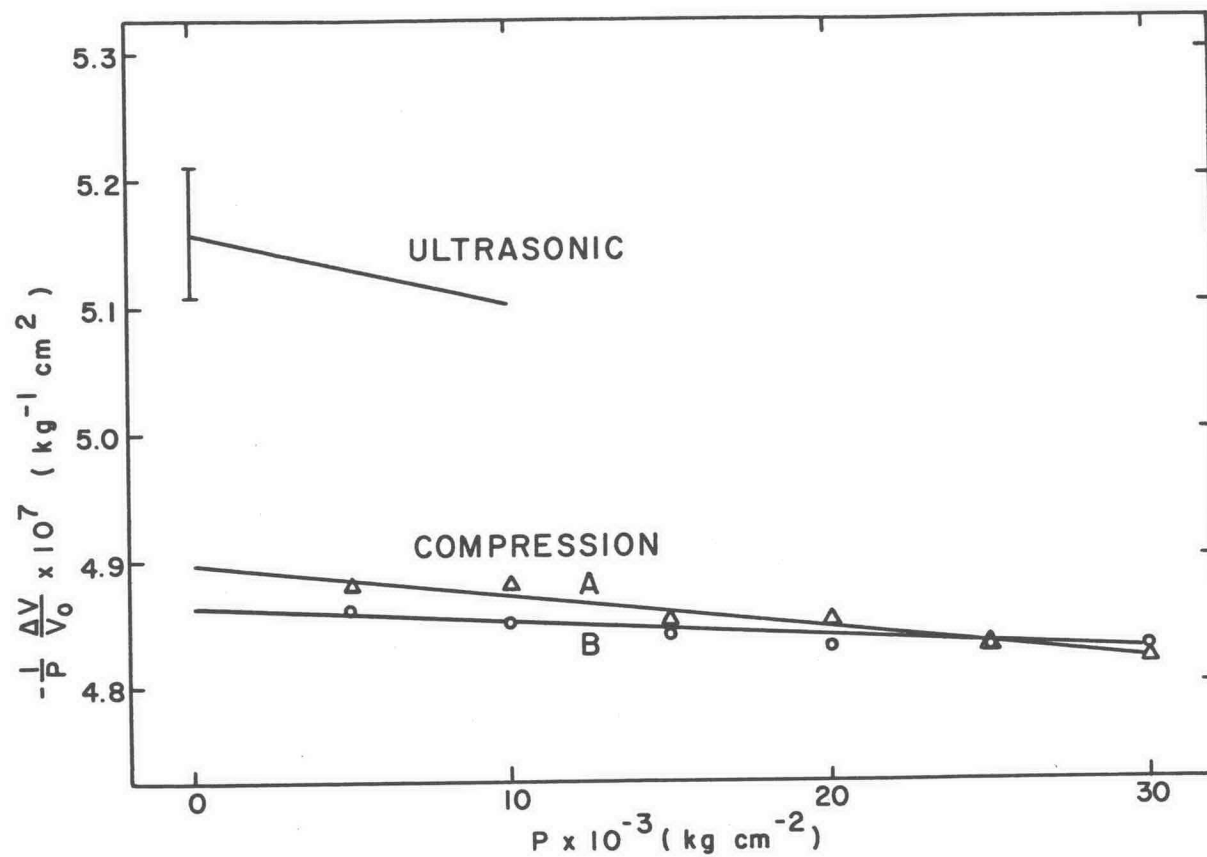
Fig. 2. Comparison between the ultrasonic and compression equations of state for tantalum. Specimens A and B are 99.9 and 99.95 + per cent purity. The error bar indicates the uncertainty of the compressibility.
